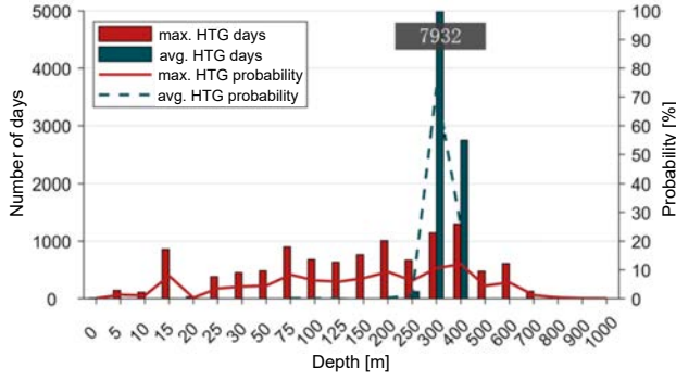
Fig. 3. Statistics and frequency distribution of the strongest depth frequency in KEF.
