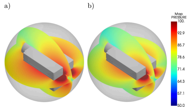
Fig. 15. Acoustic radiation slice images at fundamental frequency: a) original pump; b) improvement.
