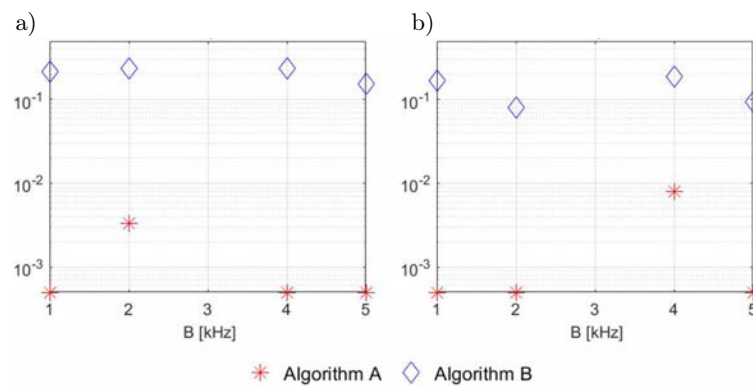
Fig. 21. The BER of the data transmission in model pool using DSSS signals constructed of m -sequences (a) and Kasami codes (b) of rank 8.
