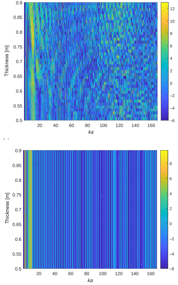
Fig. 10. Calculation of TS of a thick shell sphere changing with coupling layer thickness: a) water filling; b) air filling.
