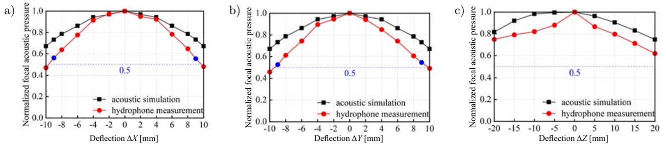
Fig. 5. Illustration of the normalized focus acoustic pressure levels deflected on the X-axis (a), the Y-axis (b), and the Z-axis (c), obtained by the hydrophone measurements and the acoustic simulations.
