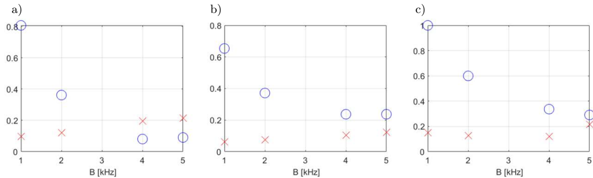
Fig. 11. The coefficients: C_A (x) and C_B (o) for transmission of DSSS signals constructed of m -sequences of rank 8 in NOF1 (a), NCS1 (b), and BCH1 (c) watermark channel.
