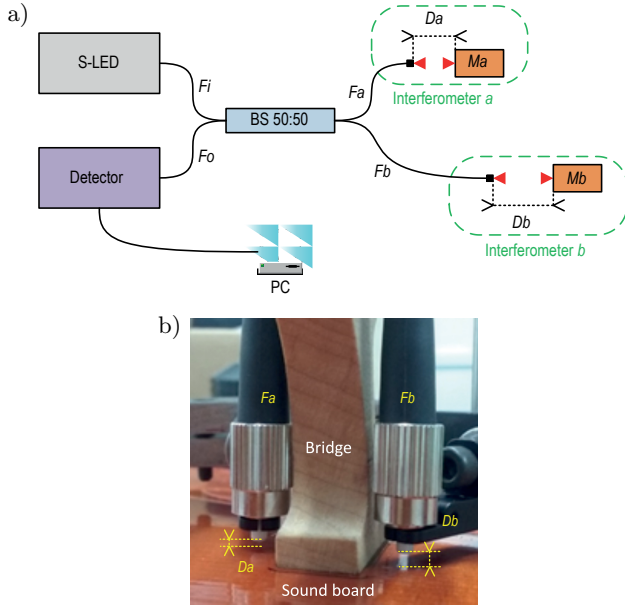
Fig. 4. (a) Interferometer schematic. The light emitted by the S-LED source is coupled to the beam splitter (BS 50:50) whose outputs, fibers Fa and Fb , illuminates the cello top plate. Da and Db are the distance between each fiber and the top plate. Beams reflected are coupled back into the fibers and sent to the detector through the fiber Fo . (b) Image of the optically instrumented cello.
