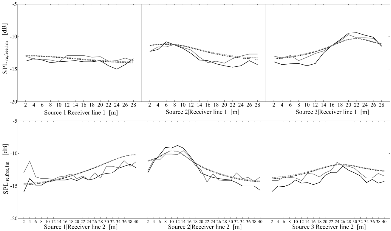
Fig. 2. SPL_{re, free, 1m} results of the hall. Solid black: experimental (HORNIX et al. , 2015); dashed black: ADM; dashed grey: SADM; and solid grey: CATT-Acoustic (HORNIX et al. , 2015).
