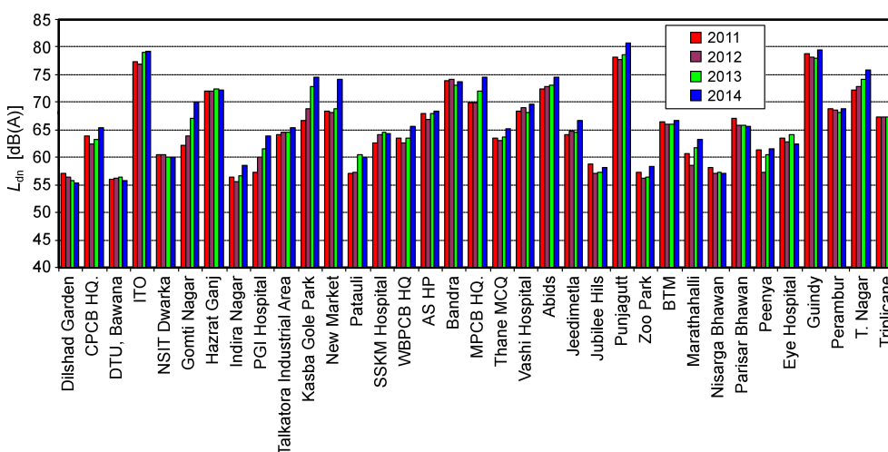
Fig. 13. L_{dn} at 35 locations spread across seven major cities all over India in year 2011–2014.
